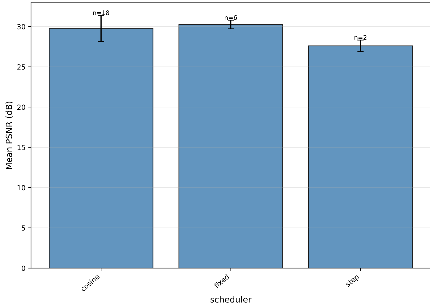
Mean PSNR per value of scheduler — OmniSR
